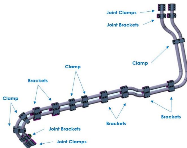
图 1-4 LOW-VS Feeder
